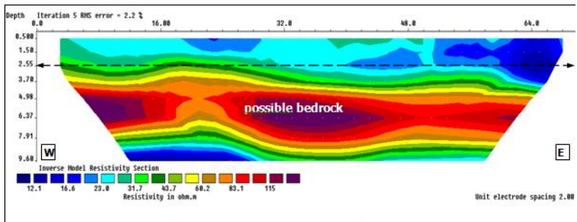
Figure 4: Pseudo section of Imaging Line 1.
